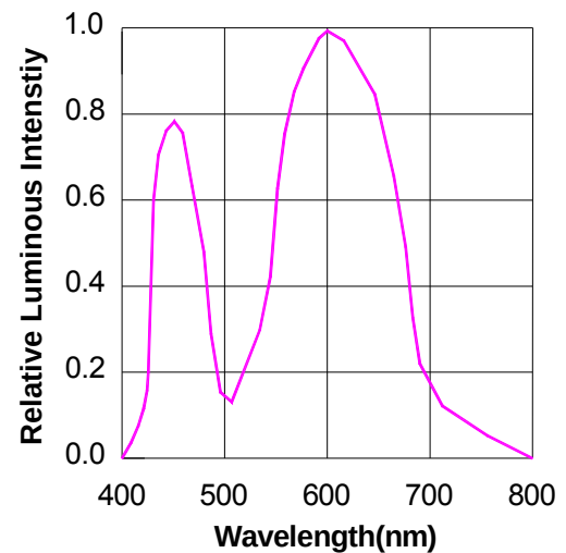
Relative Spectral Distribution, I_F=350\text{mA} , T_{Ambient}=25^{\circ}\text{C}
